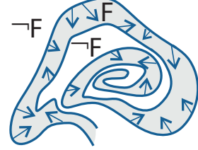
Figure 2: Differential invariant F
