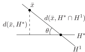
Figure 6: Illustration for the proof of Observation 5.3.
