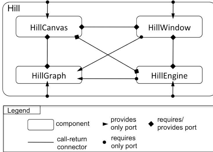
Figure 11: Partial HillClimber Architecture
