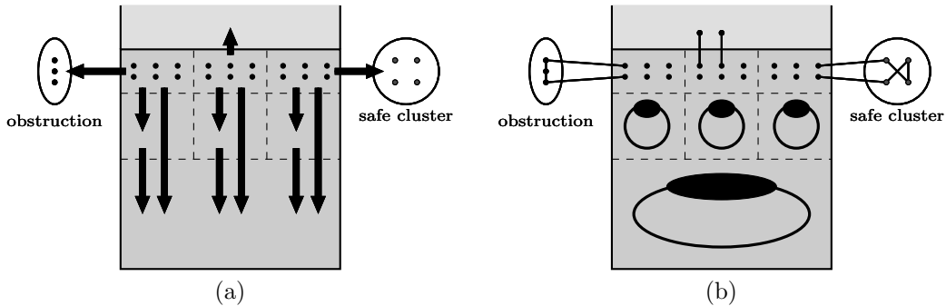
Figure 8: A schematic for the mini-games for Maker's Hamilton strategy in a good cell. (a) The marked vertices (top row) are designated to make paths through nearby obstructions and safe clusters, and to connect to good cells that are adjacent in the tree \mathcal{T} . The unmarked vertices (bottom two rows) are partitioned into subsets for blob cycle creations. Maker claims half the edges from each vertex to each lower level. (b) After all edges have been claimed, Maker has paths through obstructions and two independent edges to nearby good cells, and some unused marked vertices, and a soup of blob cycles. The blob cycles absorb the paths and unused vertices (using the many edges down to the lower levels in the good cell), culminating in the Hamilton cycle.
