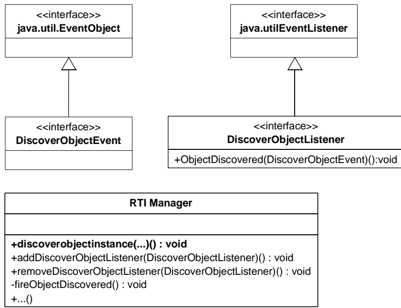
Figure 7: Event Generator Example
