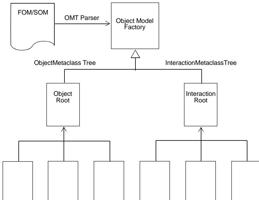
Figure 6: Object Model Factory
