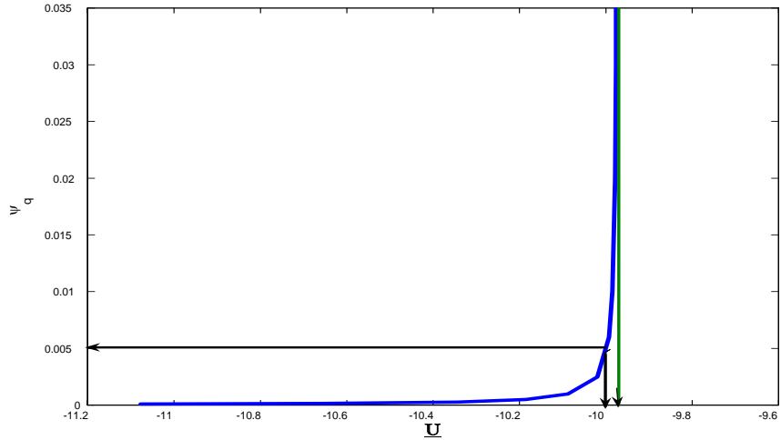
Figure 1: \psi_q and \underline{U} .
