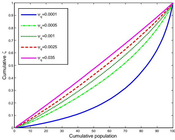
Figure 4A: Lorenz curve, \zeta
