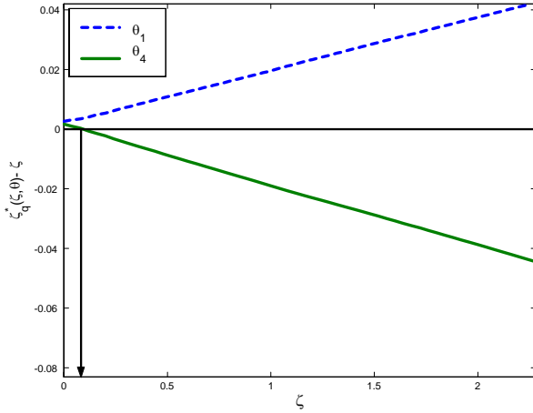
Figure 2A: \zeta_q^*(\zeta, \theta) - \zeta , \psi_q = 0.024 .
