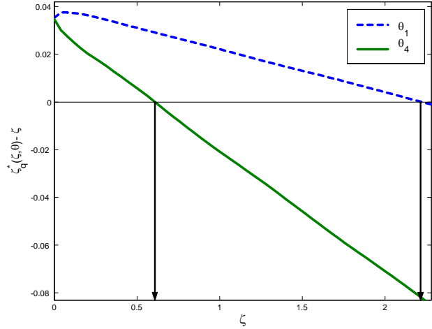
Figure 2B: \zeta_q^*(\zeta, \theta) - \zeta , \psi_q = 0.035 .
