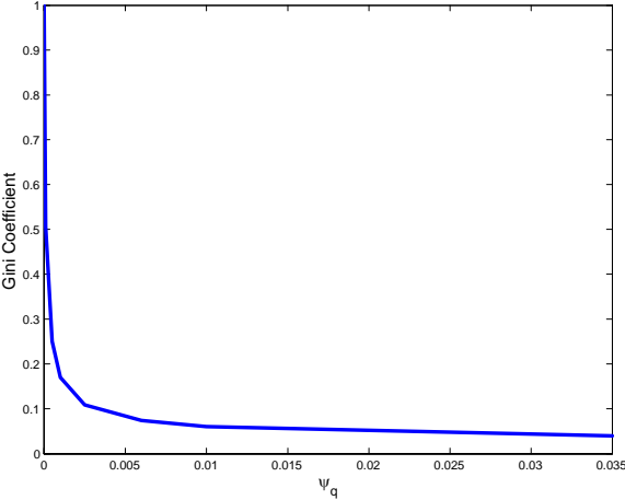
Figure 5A: Gini coefficient, \zeta
