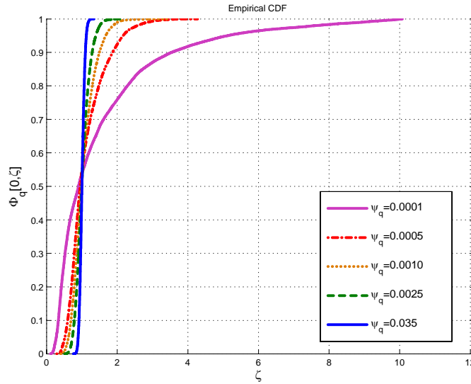
Figure 3: CDFs
