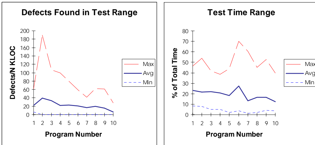
Figure 10: Unit Test Defect Density and Unit Test Time
