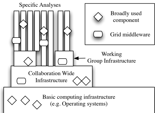
Fig. 1. A sketch of the scientific software ecosystem.
