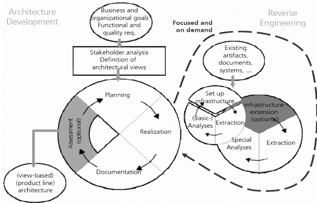
Figure 7-1: Overview PuLSE-DSSA and ADORE
