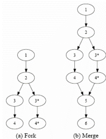
Figure 5-1: Forks and merges in an execution trace
