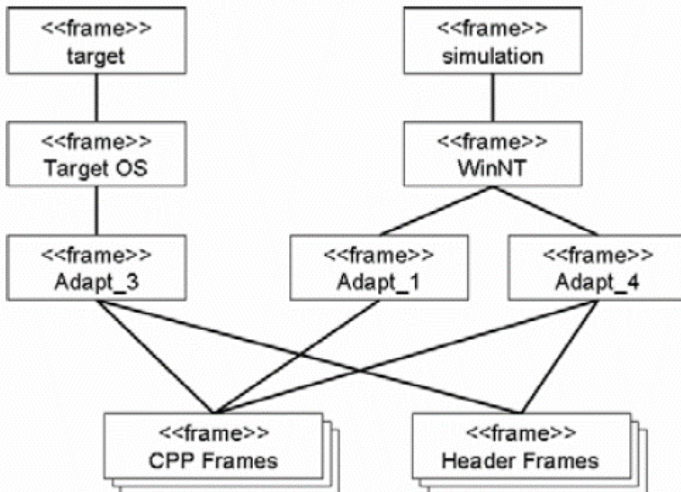
Figure 7-3: Frame Hierarchy
