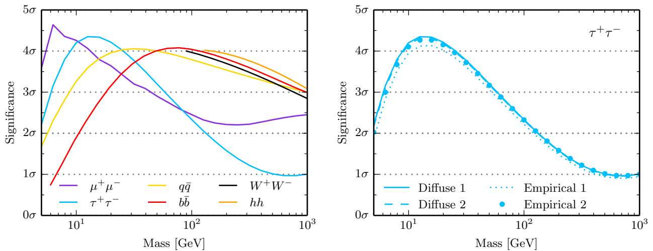
FIG. 2: Significance of the \gamma -ray excess in the direction of Reticulum II as a function of dark matter particle mass. Left: Curves correspond to the result of the search in various channels (i.e. using different ways of weighting events) using background model Diffuse 1. The curve for e^+e^- is similar to \mu^+\mu^- , ZZ is similar to W^+W^- , and q represents u, d, c, s quarks and gluons. Right: Significance in the \tau^+\tau^- channel for four different background models (see text).
