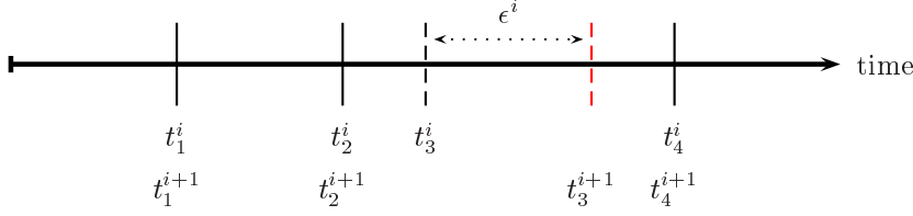
FIG. 3.1. The figure shows two runs of MST in two consecutive iterations i and i+1 . The horizontal line is the time axes while the vertical lines denote the times at which different edges become tight and are included. In the i th run edge e_i becomes tight at time t_j^i . In this example, edge e_3 is the only edge incident to a vertex of normalized degree at least d^i . Its length increases and the time at which it becomes tight during MST's execution is postponed by \epsilon^i time units.
