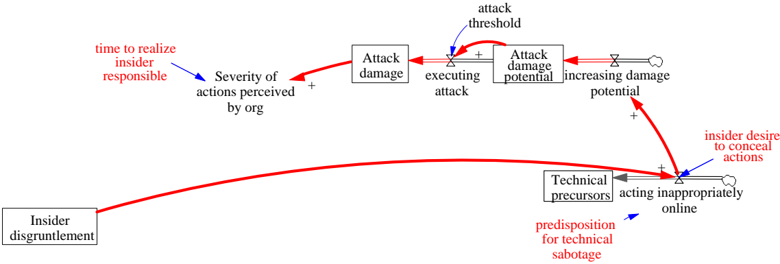
Figure 12: Attack Escalation
