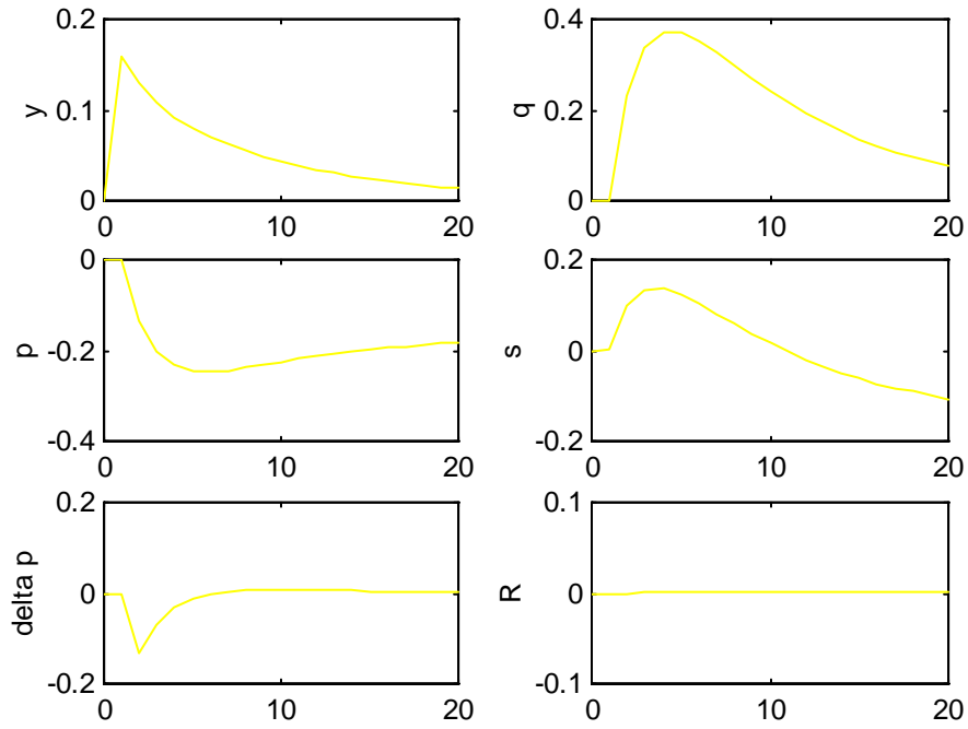
2A: Responses to Unit Shock to IS; \mu_1=1.0 , \mu_2=1.0
