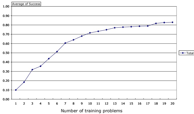
Fig. 3. Overall performance improvement in terms of the average ratio of successful model-tracing aggregated across all validation sessions and the (eight) skills. The x-axis shows the number of training problems.
