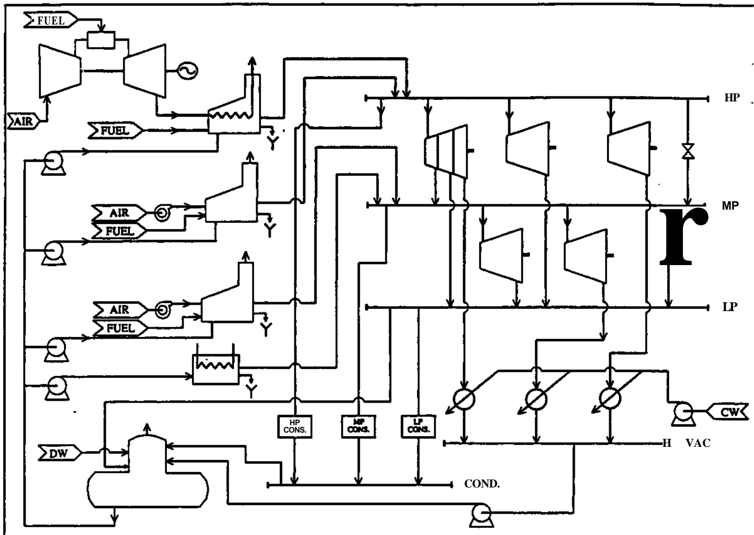
Figure 1. Superstructure of the utility plant
