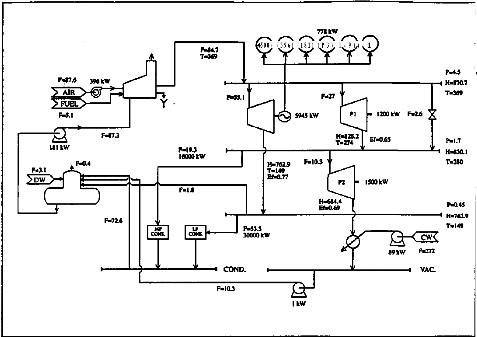
Figure 5. Optimal utility plant for example 1 with lower heating demands.
