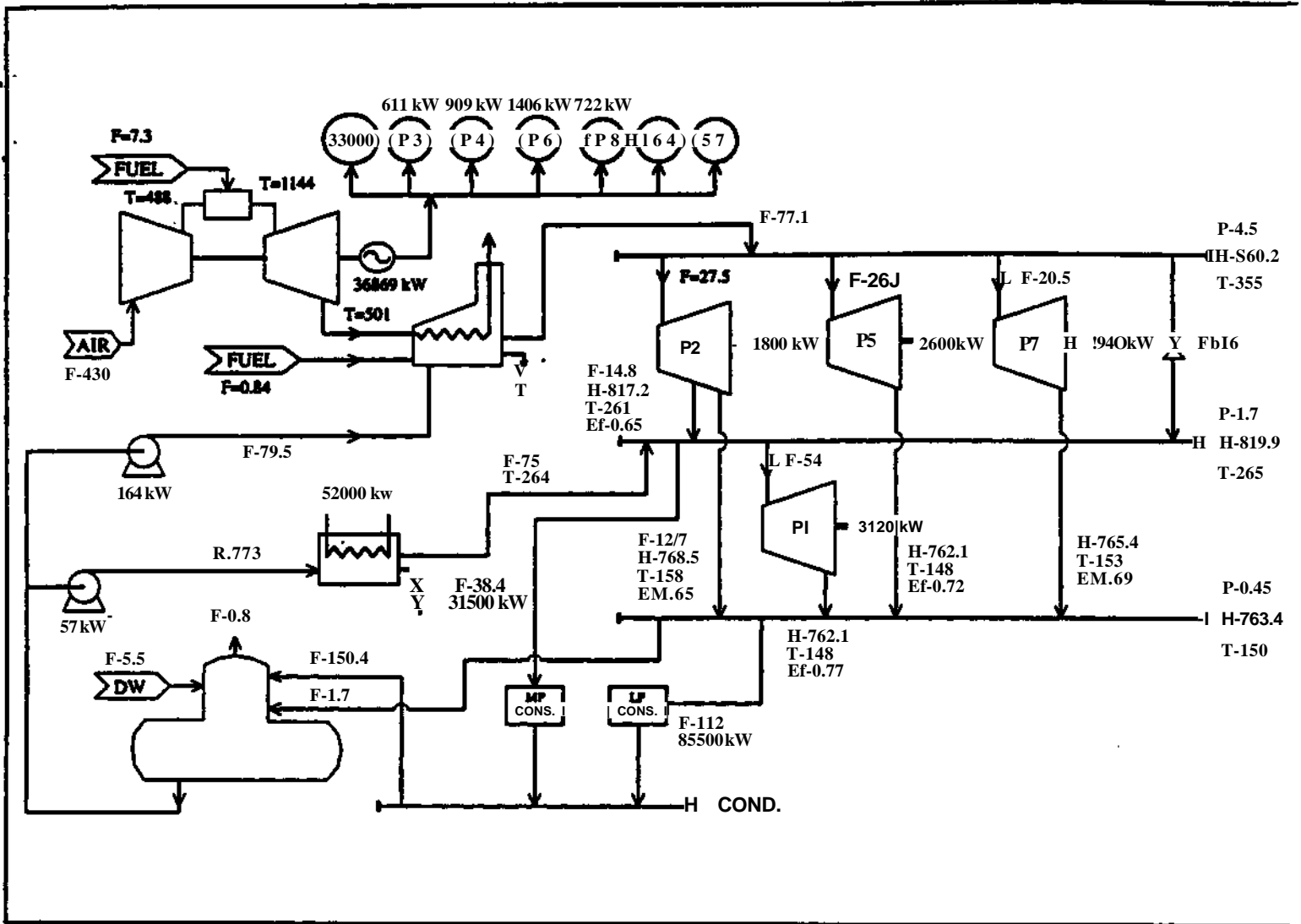
Figure 6. Optimal utility plant for example 2.
