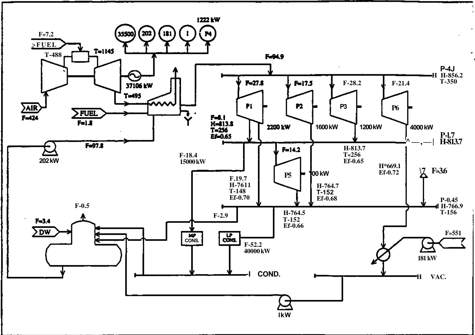
Figure 7. Optimal utility plant for example 3
