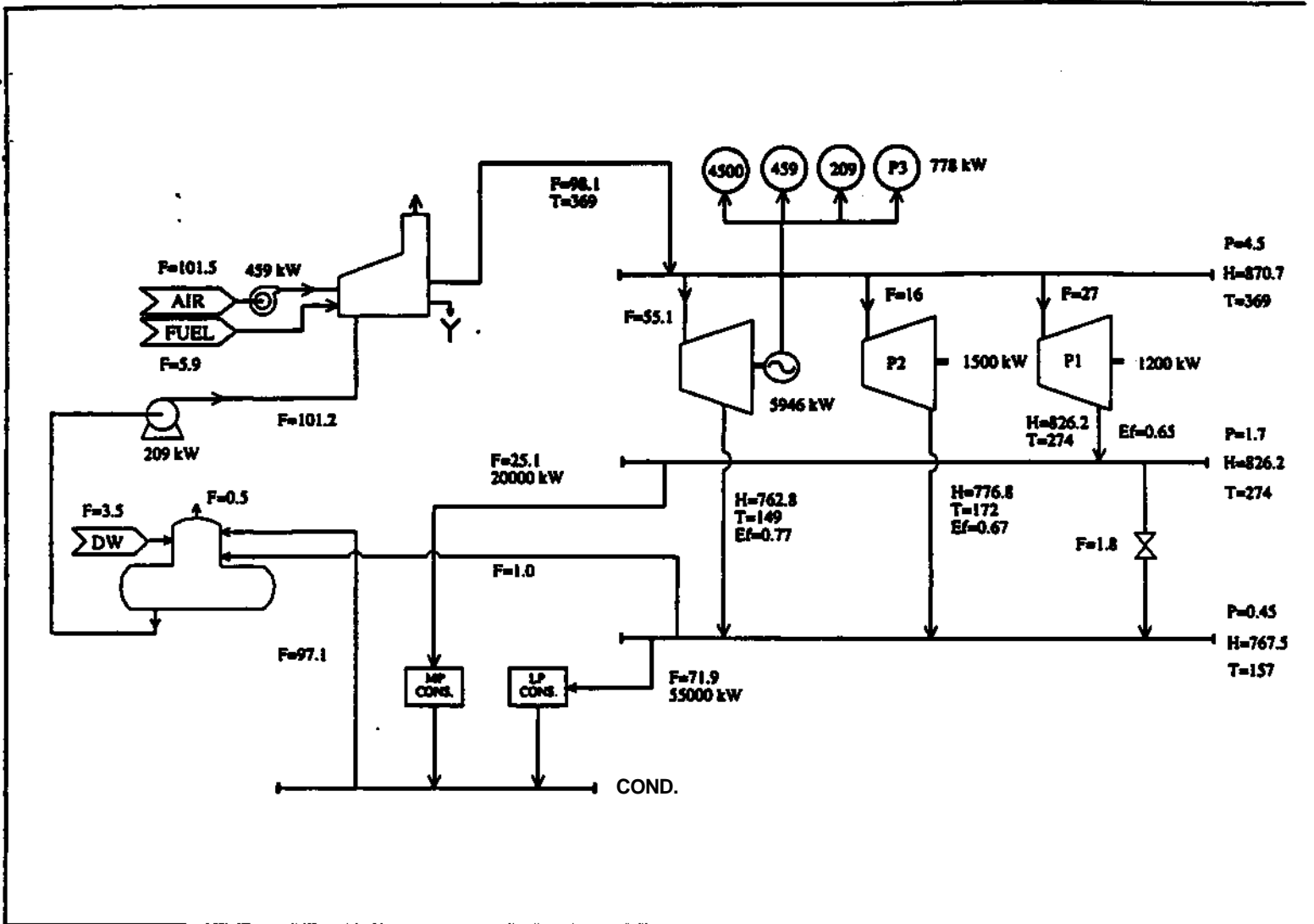
Figure 4. Optimal utility plant for example 1
