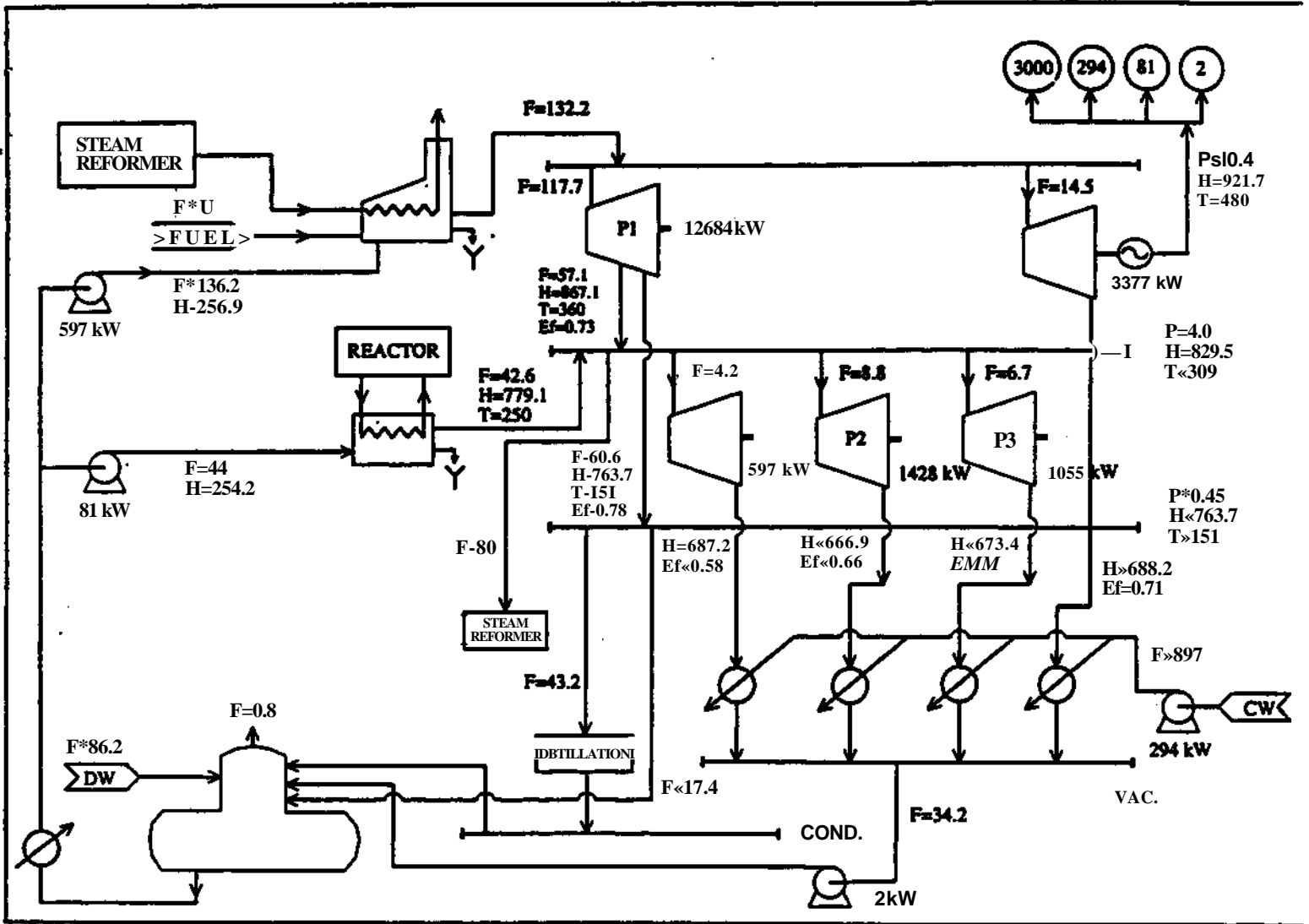
Figure 8. Optimal utility plant for example 4
