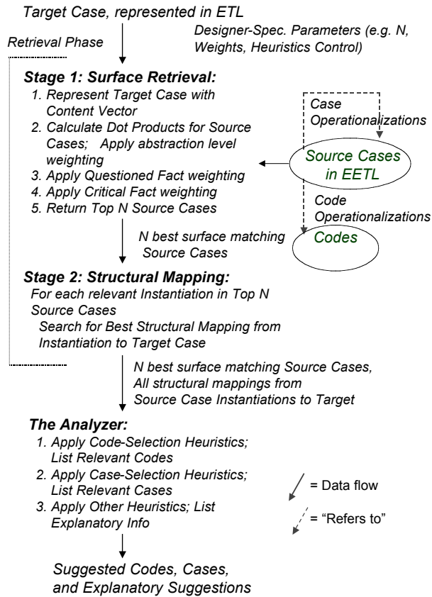
Figure 5: SIROCCO's Algorithm
