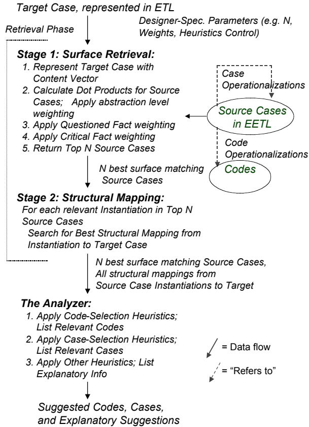
Figure 5: SIROCCO's Algorithm
