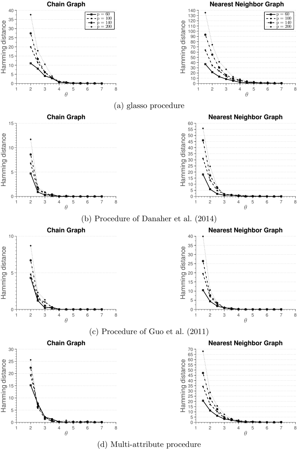
Figure 3: Results of Simulation 2 described in Section 5.1. Average hamming distance plotted against the rescaled sample size. Blocks \Omega_{ab} of the precision matrix \Omega are diagonal matrices.
