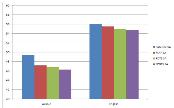
Figure 1: Cross-entropy of the adaptation data for various models
