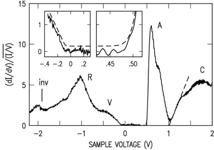
FIG 1. Tunneling spectrum of the Ge(111)c(2×8) surface, acquired at 61 K. Insets show fitting of the onsets of the valence band and of the adatom surface-band, to a function that assumes linear onset behavior modified by effects of temperature and modulation voltage.
