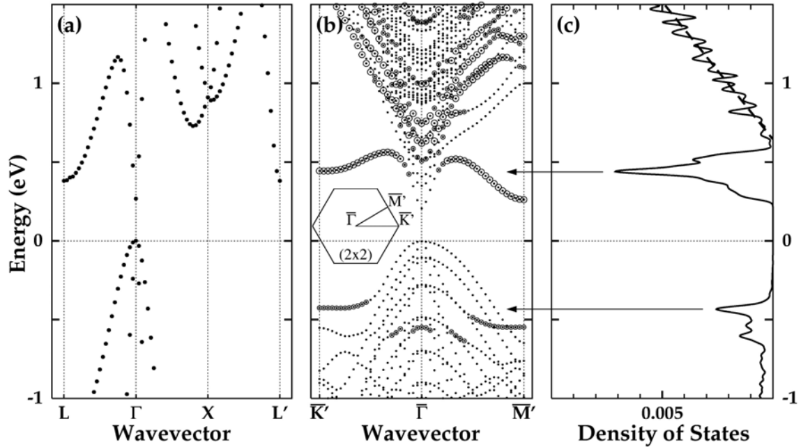
FIG 2. (a) Bulk band structure of Ge along the symmetry lines connecting L=2\pi/a(1/2,1/2,1/2) , X=2\pi/a(0,0,1) , and L'=2\pi/a(-1/2,-1/2,+1/2) . The bulk lattice constant, a , was calculated as 0.578 nm. (b) Surface band structure of Ge(111)2×2: Large and medium open circles represent surface localized states containing more than 0.02% and 0.01%, respectively, of charge in the surface region of 0.45 – 0.55 nm away from the ideal first layer. (c) Surface density of states of Ge(111)2×2 obtained by integrating the local density of states over the surface region of 0.45 – 0.55 nm away from the ideal first layer. Arrows indicate the band-state origins of the state-density peaks. All energies are given relative to the VBM.
