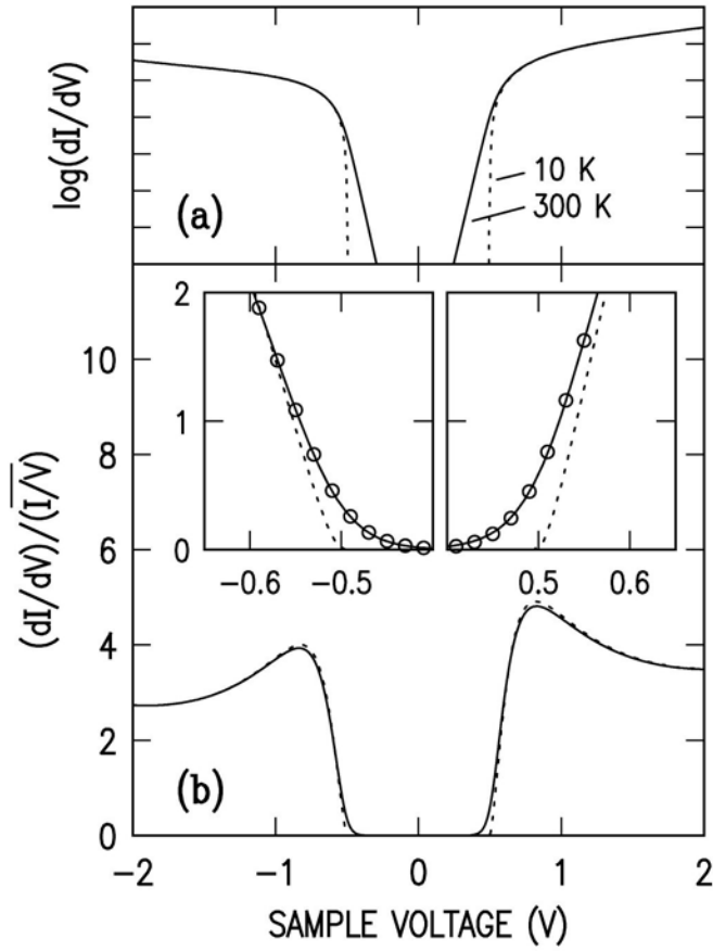
FIG 8. Simulation of tunneling spectra for tunneling into effective mass bands, with onsets at \pm 0.5 V. The computed spectra are displayed as (a) conductance at constant sample-tip separation (one decade per division) and (b) normalized conductance on a linear scale, and results are shown for temperatures of 10 K (dotted lines) and 300 K (solid lines). The insets in (b) show an expanded view of the band onsets, with circles indicating a fit to the 300 K onset using a functional form that includes the temperature dependence of the normalized conductance.
