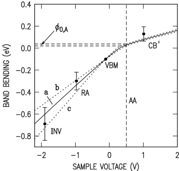
FIG 4. Band bending in the semiconductor at a point opposite the probe tip apex, as a function of sample-tip voltage. Data points are shown for spectral features that have known energy such that the band bending can be absolutely determined (VBM – valence band maximum, RA – peak of rest-atom band, CB' – high lying conduction band feature, and INV – voltage at which inversion occurs). Theoretical curves interpolating between the data points are shown, with the solid line giving a typical result and the dotted lines giving maximal results consistent with the data. The vertical dashed line is located at the position of the observed onset of the adatom band (AA), with the horizontal dashed lines then giving the band bending at this voltage.
