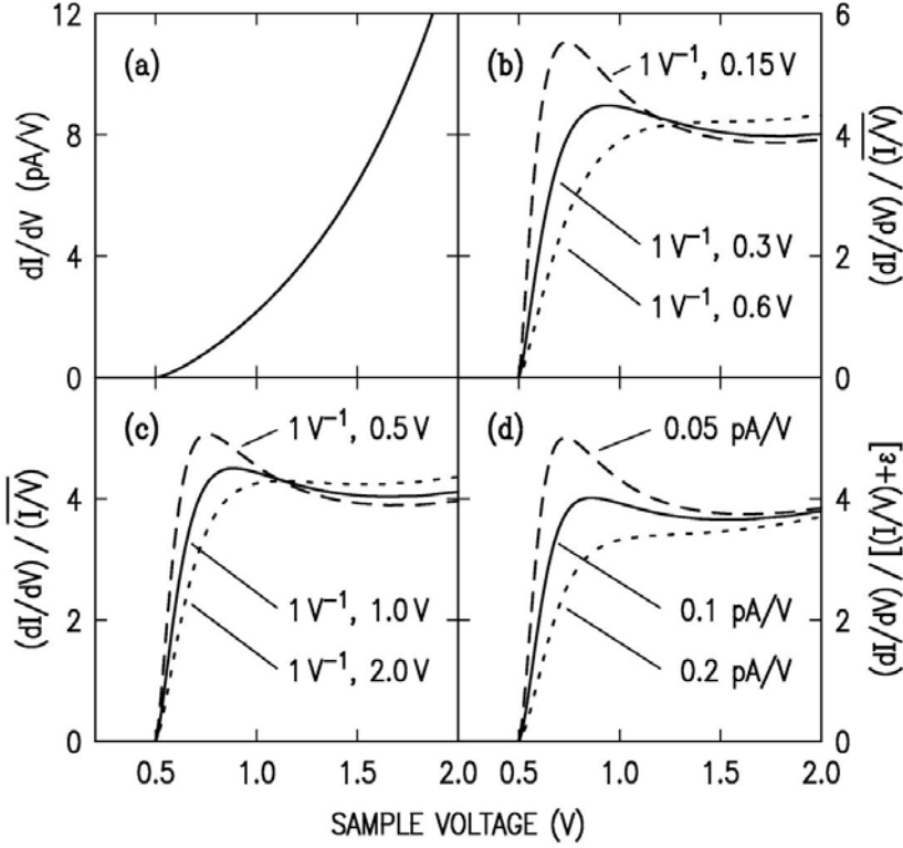
FIG 7. Comparison of various methods for spectroscopic normalization: (a) Simulated curve of dI/dV based on tunneling at a temperature of 10 K into an effective-mass band with onset at +0.5 V. (b) Normalization performed by convolution of I/V with exponential function, for the values of a' and \Delta V' indicated. (c) Normalization performed by convolution of I/V with function composed of sine- and cosine-integrals, for the values of a' and \Delta V indicated. (d) Normalization performed by addition of a constant to I/V , for the values of \varepsilon indicated.
