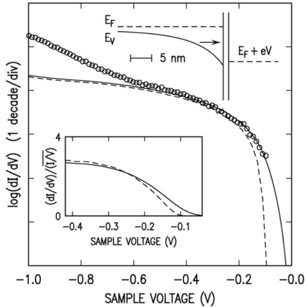
FIG 6. Conductance at constant sample-tip separation for the spectral region near the VBM, comparing simulated results with (solid line) and without (dashed line) quantum effects, along with experimental data (open circles). The lower inset shows computed (dI/dV)/(I/V) curve for the simulated results. The upper inset shows the potential profile from the simulations at a sample-tip voltage of -0.111 V, with the arrow indicating the transmission through the semiconductor depletion region that is included in the quantum simulations.
