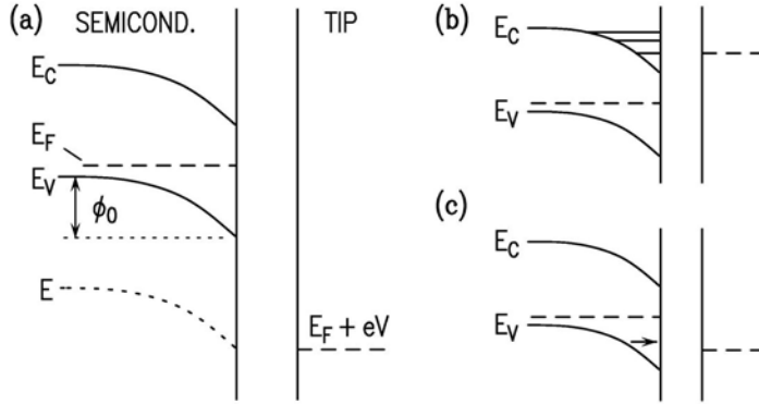
FIG 3. (a) Sketch of energy bands used for computations of the electrostatic potential. The sample Fermi-level is denoted by E_F with the tip Fermi-level at E_F + eV where V is the sample-tip voltage. The band bending at the surface is denoted by \phi_0 , with V and \phi_0 both being negative in this diagram. Quantum effects within the semiconductor can produce shifts in the observed band edges, as illustrated in (b) and (c) for localized state formation and for wavefunction tailing through a depletion region, respectively.
