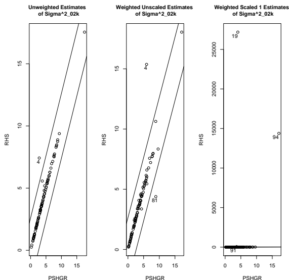
Figure 20: Comparison of PSHGR vs. RHS for Estimates from Equation 23
