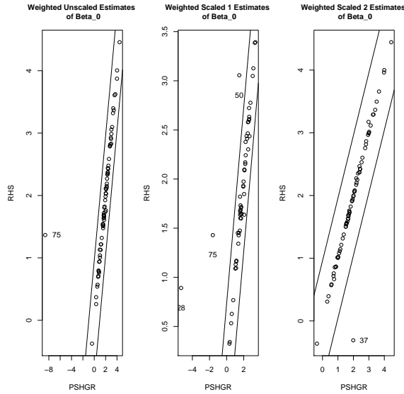
Figure 31: Comparison of PSHGR vs. RHS for Estimates of \beta_0 from Equation 35
