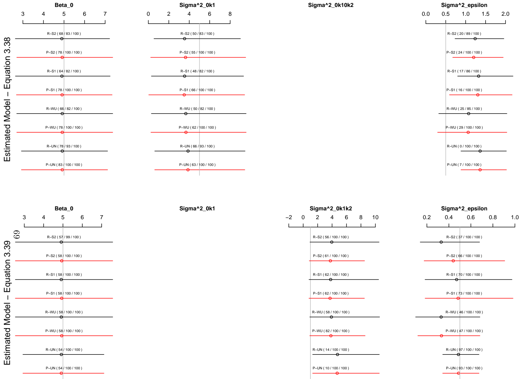
Figure 11: Results for Misspecification of Clustering Layers, Simulation Set 12 Generated Model - Equation 37
