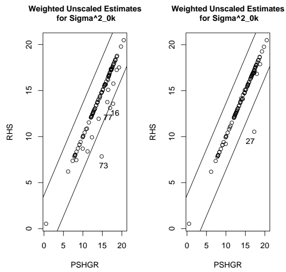
Figure 23: Comparison of PSHGR vs. RHS for Estimates from Equation 26
