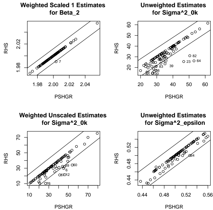
Figure 12: Comparison of PSHGR vs. RHS for Estimates from Equation 4
