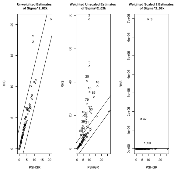
Figure 34: Comparison of PSHGR vs. RHS for Estimates of \sigma_{02k}^2 from Equation 35
