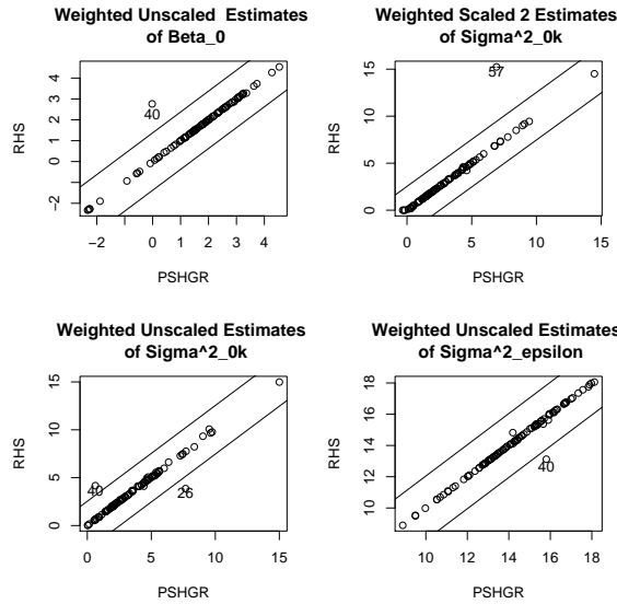
Figure 25: Comparison of PSHGR vs. RHS for Estimates from Equation 31
