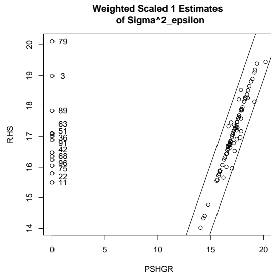
Figure 26: Comparison of PSHGR vs. RHS for Estimates from Equation 31 (cont)
