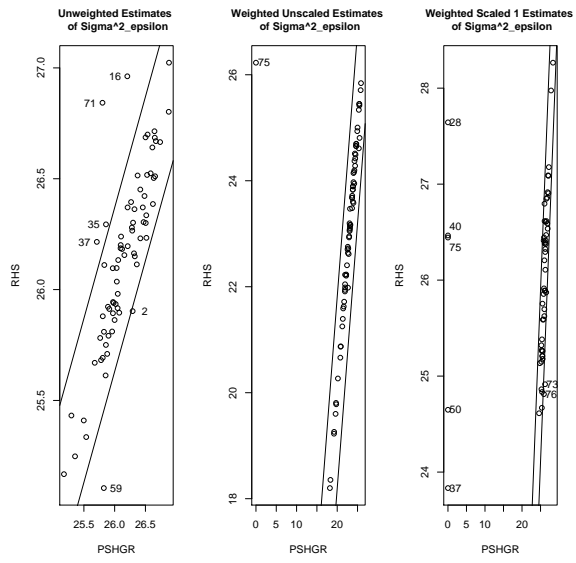
Figure 36: Comparison of PSHGR vs. RHS for Estimates of \sigma_\epsilon^2 from Equation 35
