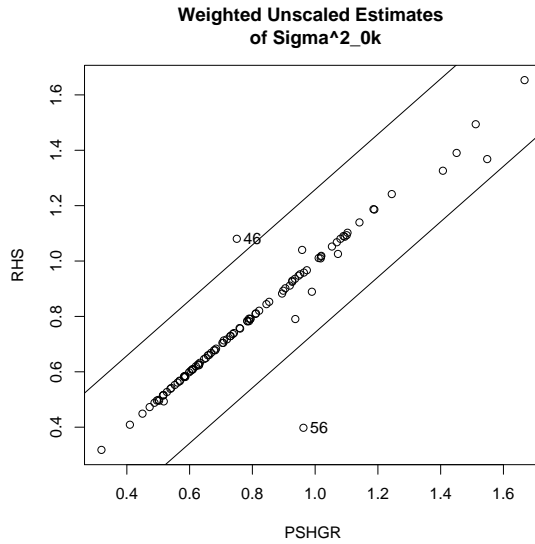
Figure 17: Comparison of PSHGR vs. RHS for Estimates from Equation 14
