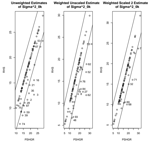
Figure 30: Comparison of PSHGR vs. RHS for Estimates from Equation 34
