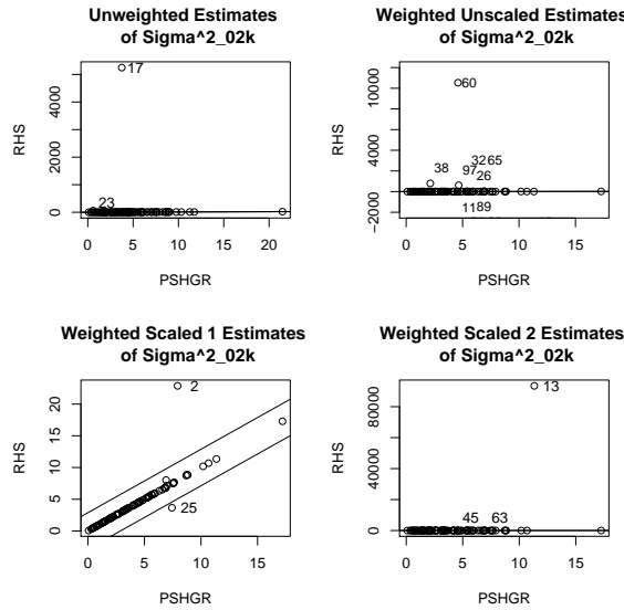
Figure 28: Comparison of PSHGR vs. RHS for Estimates of \sigma_{02k}^2 from Equation 33
