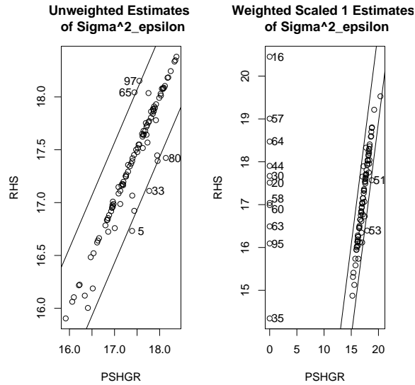
Figure 24: Comparison of PSHGR vs. RHS for Estimates from Equation 29
