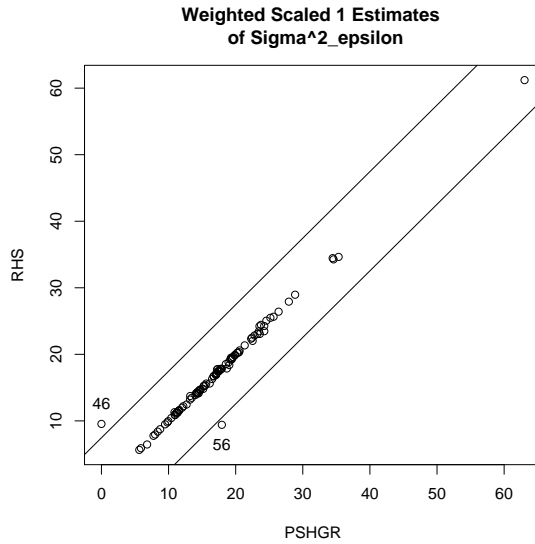
Figure 19: Comparison of PSHGR vs. RHS for Estimates from Equation 18
