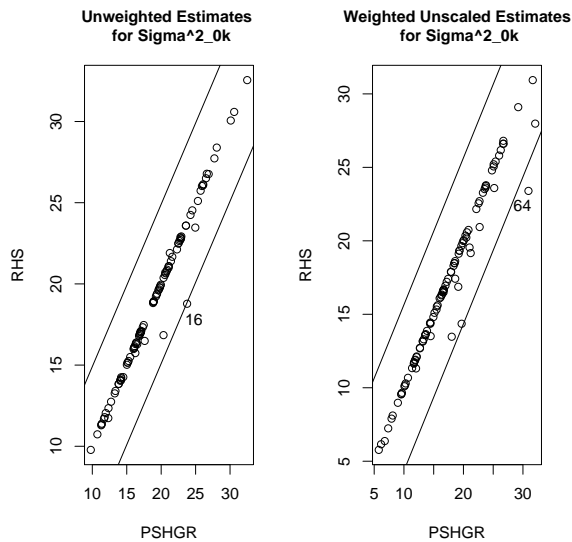
Figure 22: Comparison of PSHGR vs. RHS for Estimates from Equation 24
