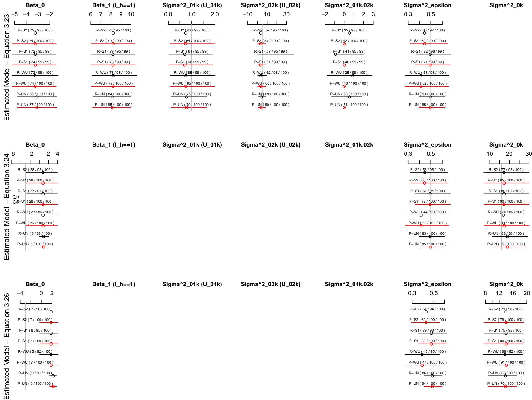
Figure 8: Results for Misspecification of Stratification Layers, Simulation Set 9 Generated Model - Equation 22
