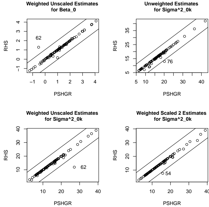
Figure 16: Comparison of PSHGR vs. RHS for Estimates from Equation 12
