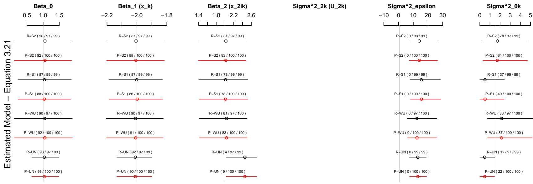
Figure 7: Results for Misspecification of Random Variables, Simulation Set 8 Generated Model - Equation 19
