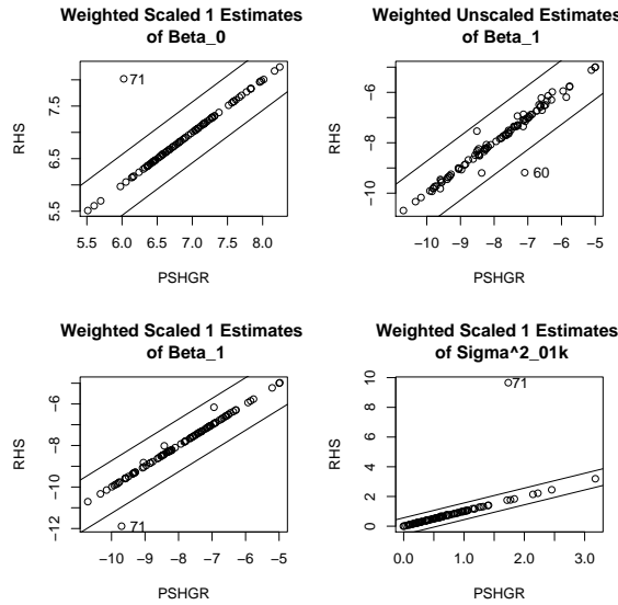
Figure 27: Comparison of PSHGR vs. RHS for Estimates from Equation 33
