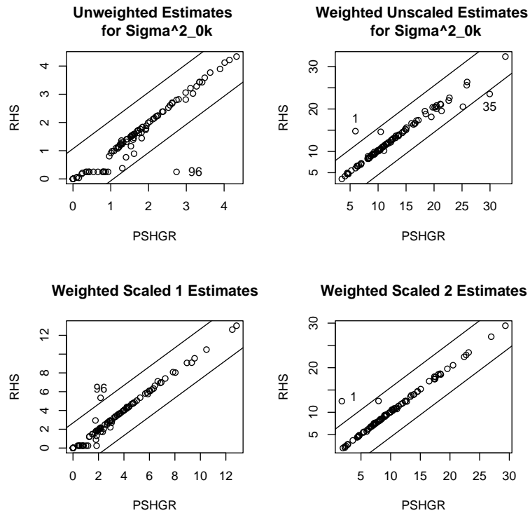
Figure 15: Comparison of PSHGR vs. RHS for Estimates from Equation 9
