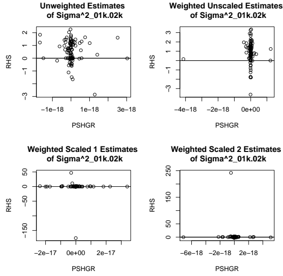
Figure 29: Comparison of PSHGR vs. RHS for Estimates of \sigma_{01k.02k}^2 from Equation 33
