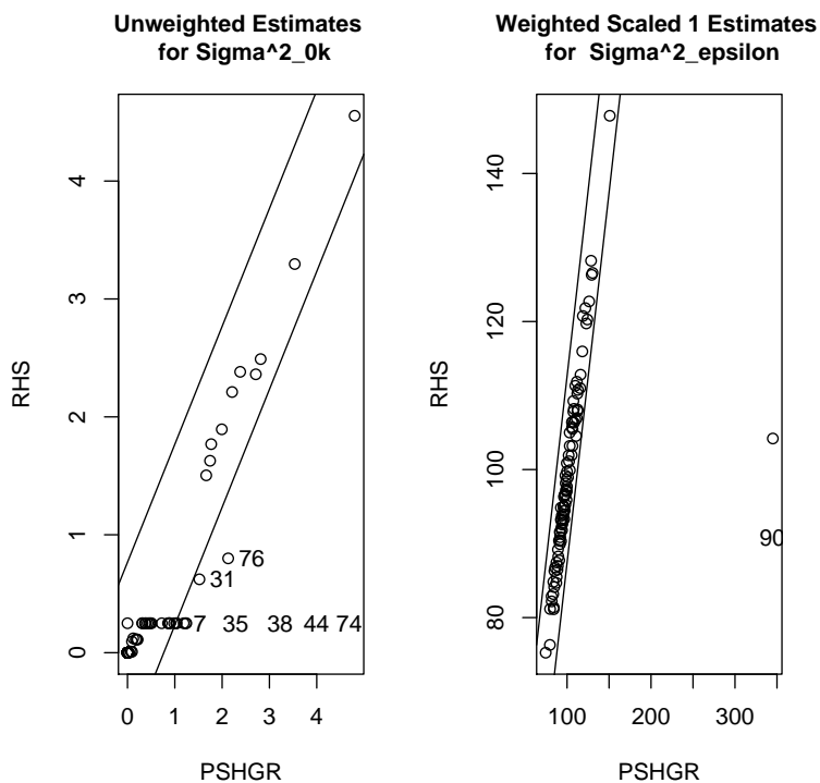
Figure 13: Comparison of PSHGR vs. RHS for Estimates from Equation 5
