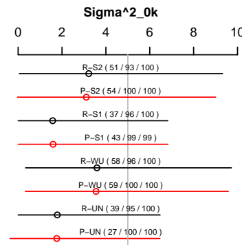
Figure 9: Results for Misspecification of Stratification Layers, Simulation Set 10 Generated Model - Equation 27
