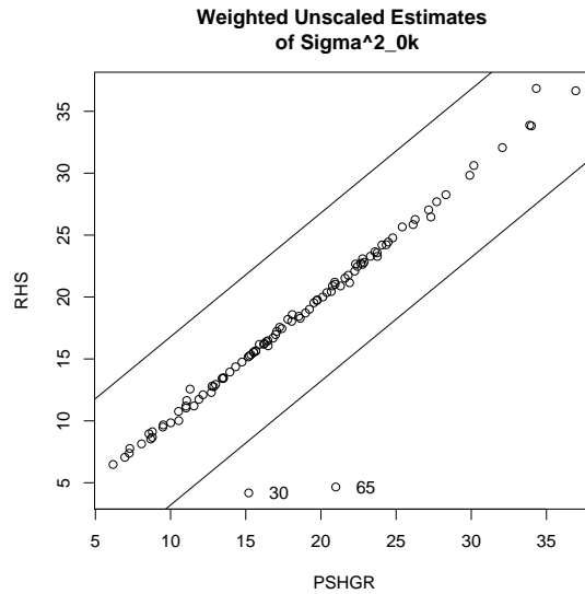
Figure 37: Comparison of PSHGR vs. RHS for Estimates of \sigma_{0k}^2 from Equation 36
