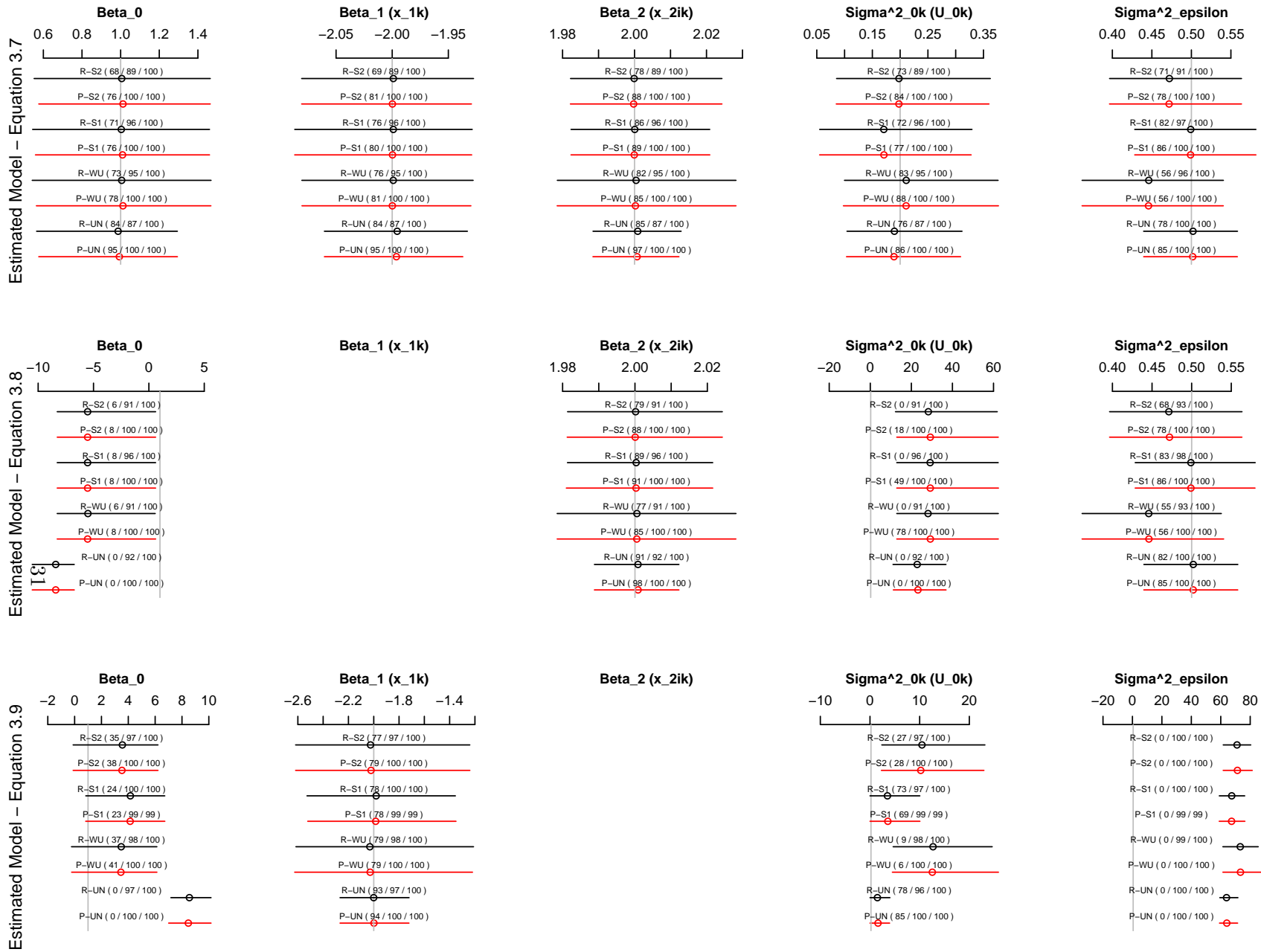
Figure 3: Results for Misspecification of Fixed Effects, Simulation Set 4Generated Model - Equation 6
