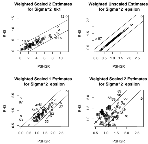
Figure 38: Comparison of PSHGR vs. RHS for Estimates from Equation 38
