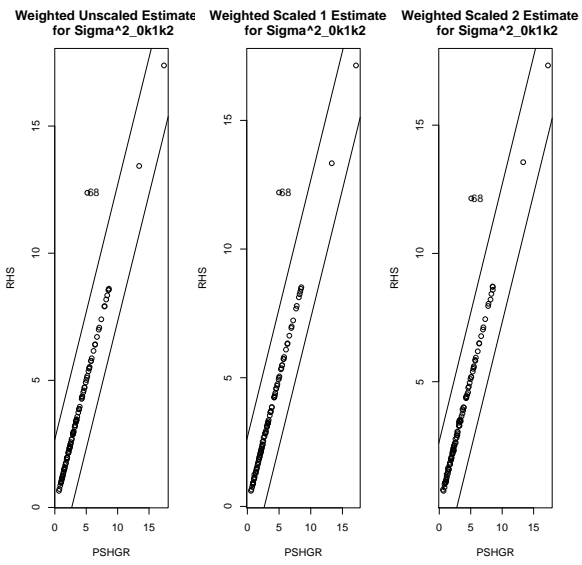
Figure 39: Comparison of PSHGR vs. RHS for Estimates from Equation 39
