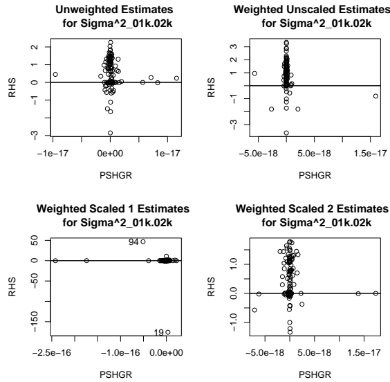
Figure 21: Comparison of PSHGR vs. RHS for Estimates of \sigma_{01k.02k}^2 from Equation 23
