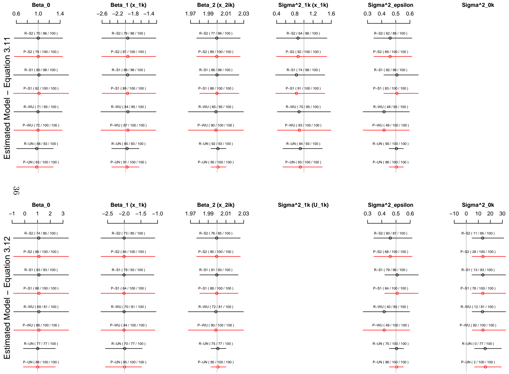
Figure 4: Results for Misspecification of Random Variables, Simulation Set 5 Generated Model - Equation 10
