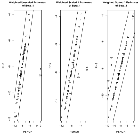
Figure 32: Comparison of PSHGR vs. RHS for Estimates of \beta_1 from Equation 35
