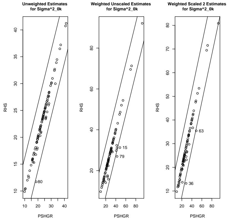
Figure 14: Comparison of PSHGR vs. RHS for Estimates from Equation 8
