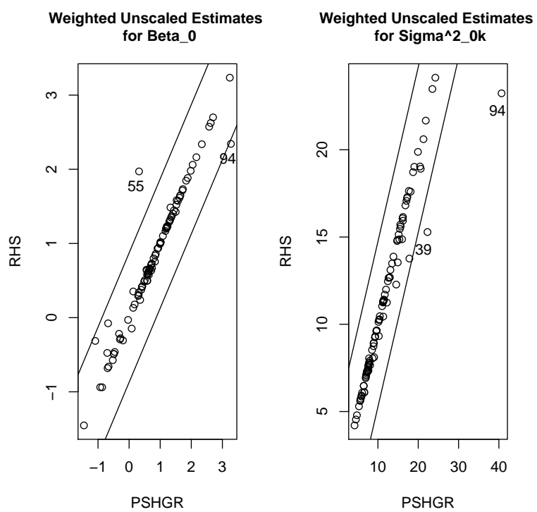
Figure 18: Comparison of PSHGR vs. RHS for Estimates from Equation 15
