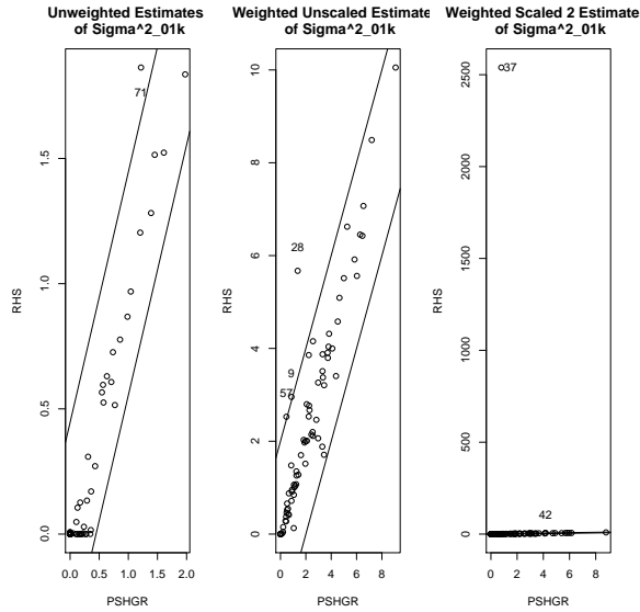
Figure 33: Comparison of PSHGR vs. RHS for Estimates of \sigma_{01k}^2 from Equation 35
