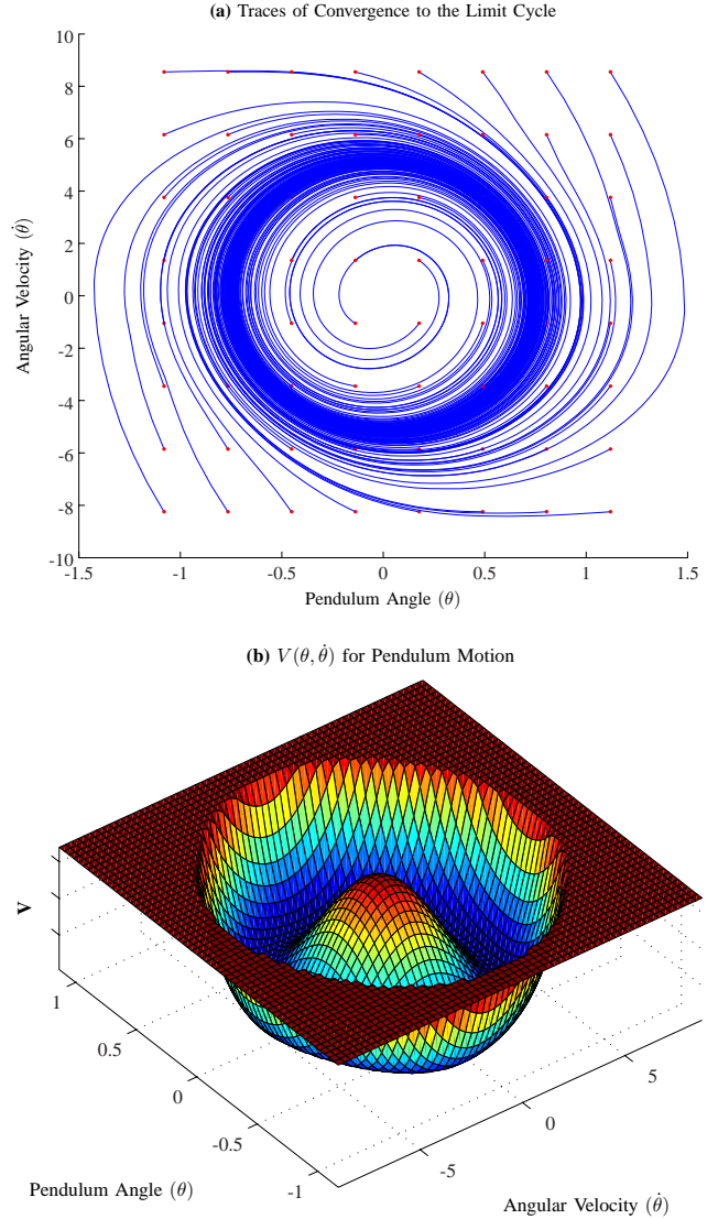
Fig. 2. (a) Traced trajectories of DP controlled motion from various points in the pendulum state space. (b) The pendulum value function shows a valley at the limit cycle.
