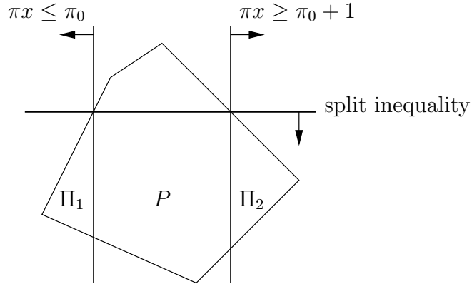
Figure 6: A split inequality
