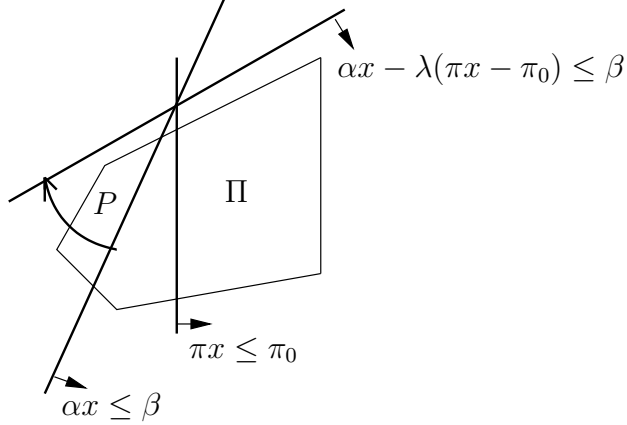
Figure 8: Illustration of Lemma 5.3
