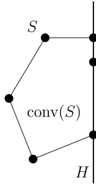
Figure 10: Illustration of Lemma 7.3
