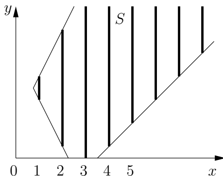
Figure 1: A mixed integer set
