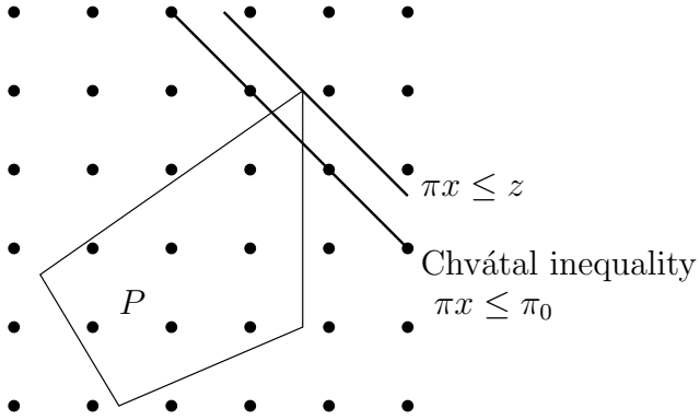
Figure 7: Chvátal inequality
