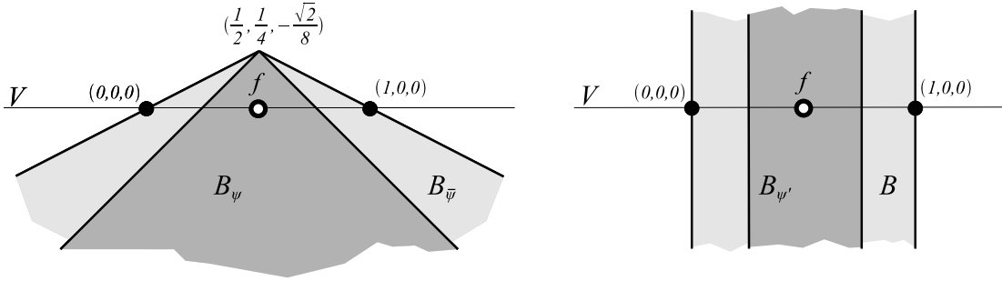
Figure 2: Lattice-free sets in the 2-dimensional space W .
