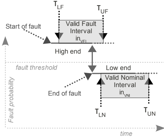
Figure 4: Diagram of the thresholds used to determine tolerances of the wave shape.
