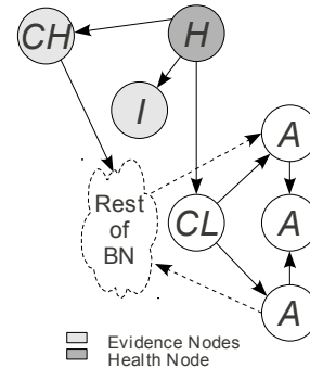
Figure 6: External diagnosis BN model of a typical load (component) using intermittent diagnosis via the intermittent node I .
