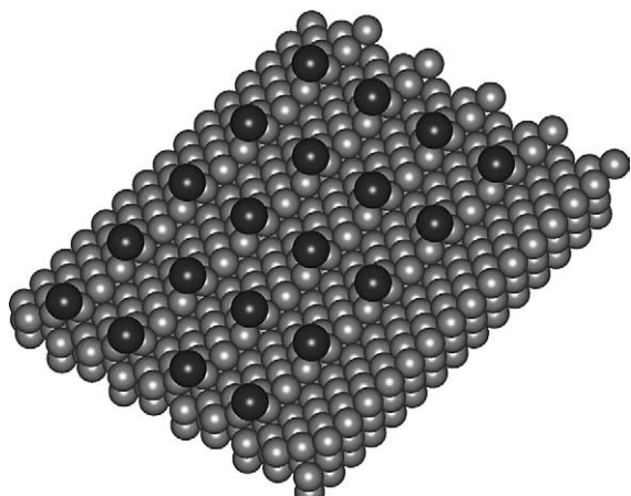
Fig. 1. The Cu(221) surface has (111) terraces that are three atomic distances in width separated by monoatomic (110) steps. The model of the Cu(221) surfaces illustrates a single iodine atom adsorbed at the top of the step edge as predicted by DFT calculations.
