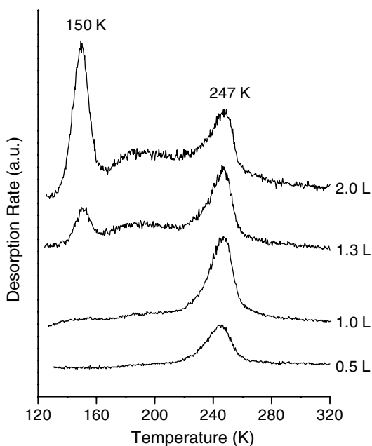
Fig. 2. TPD spectra of ethyl iodide adsorbed at 100 K on Cu(111) using various exposures. The peak at 247 K arises from ethylene desorption while the peak at 150 K is due to the desorption of molecular ethyl iodide. The appearance of the ethyl iodide desorption peak after an exposure of 1.3 L indicates that the ethyl iodide monolayer is saturated by an exposure of \sim 1.0 L. Ethyl groups on the surface undergo \beta -hydride elimination to produce ethylene desorption at 247 K. The fragment monitored was m/q = 27 ( C_2H_3^+ ). The heating rate was 2 K/s.
