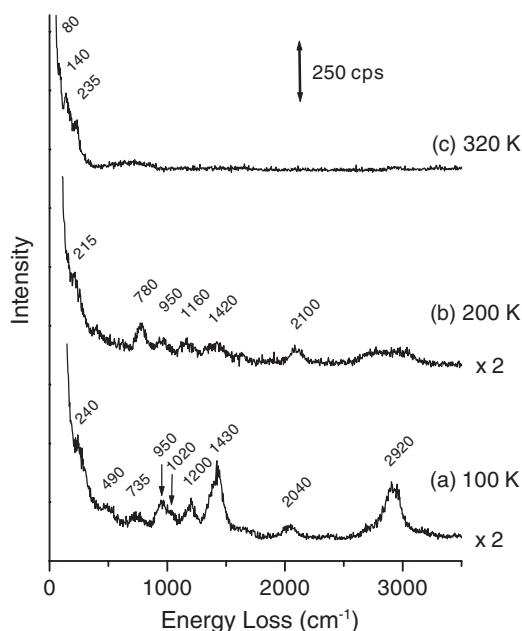
Fig. 5. HREEL spectra of the Cu(221) surface (a) after exposure to 1.0 L of ethyl iodide at 100 K, (b) after annealing to 200 K to form C_2H_5(a) and I(a) , and (c) after further annealing to 320 K to leave iodine only on the surface.
