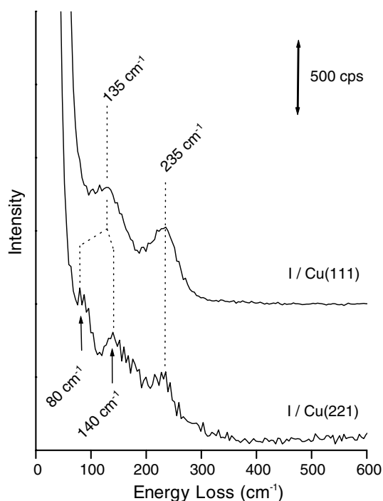
Fig. 7. HREEL spectra of iodine on the Cu(111) and Cu(221) surfaces. The 80 \text{cm}^{-1} loss peak is assigned to the vibration of iodine atoms adsorbed on the top of the step edges on the Cu(221) surface.
