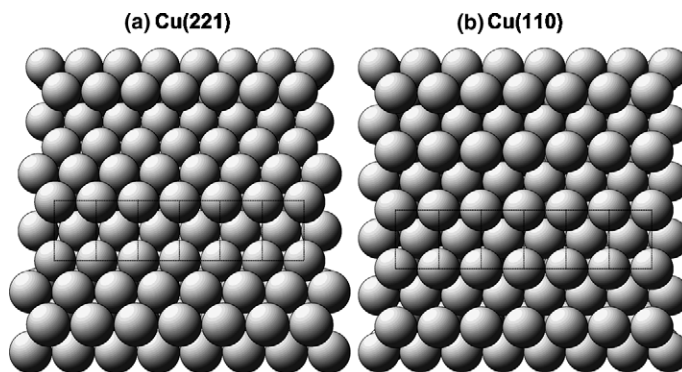
Fig. 6. Top view of the (a) Cu(221) and (b) Cu(110) surfaces. The step edge of the (221) surface has (110) structure.
