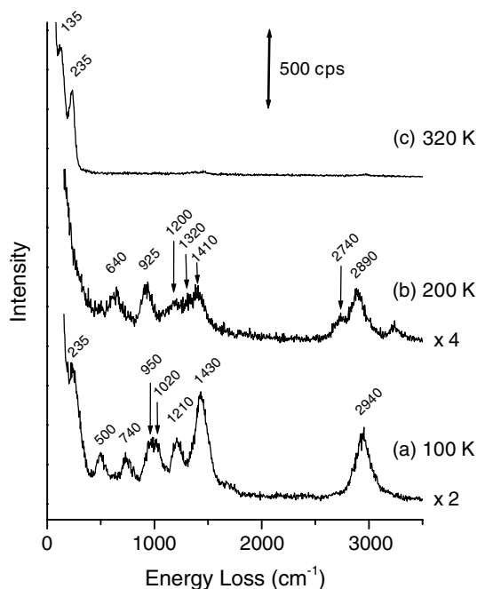
Fig. 3. HREEL spectra of the Cu(111) surface (a) after exposure to 1.0 L of ethyl iodide at 100 K, (b) after annealing to 200 K to form C_2H_{5(a)} and I_{(a)} , and (c) after further annealing to 320 K to leave iodine only on the surface.
