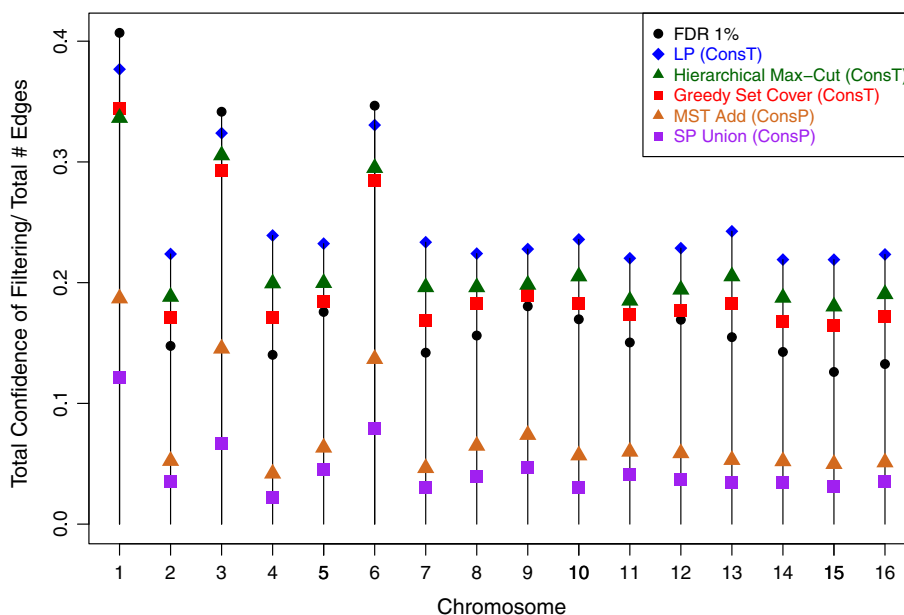
Figure 1 Metric filtering performance on various chromosomes of yeast. The total confidence that each algorithm recovers normalized by the total number of edges is plotted. Higher values are better. The objective value of the linear program (blue diamonds) gives an upper bound for both the ConsT and ConsP solutions. We also compare our algorithms to the Duan et al. filtering method at FDR 1% (black circles) which is their largest and highest-confidence filtered interaction set. (A bug in the SP-UNION script in the conference version of this paper [20] erroneously led to plotting the sum of edge q-values instead of the sum of confidence. The plots have been updated to correctly plot total confidence with little qualitative difference).
