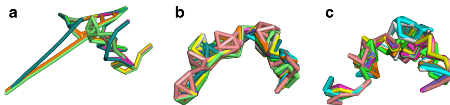
Figure 2 Filtered graphs embedded in 3D. Superposition of 10 embeddings for both ConsT and C-RANK filterings. (a) SET-COVER . (b) C-RANK of the same size as the SET-COVER . (c) SET-COVER after removing \approx 20\% of the lowest-confidence edges.
