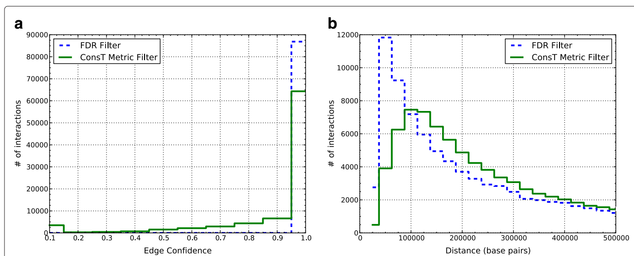
Figure 3 Histogram of genomic distances and interaction confidences between C-Rank and ConstT. Distances and confidences for both filtering methods were computed on the intra-chromosomal interactions. (a) The ConstT filtering kept more low-confidence edges than C-Rank ("FDR Filter" in the legend). (b) The ConstT filtering kept interactions with larger genomic distances than C-Rank.
